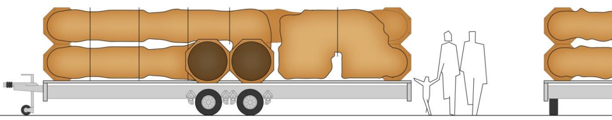
Trailer and caving system - Ready for transportation
